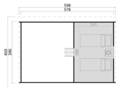
MURANO 3 UPPER FLOOR
