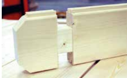
Wind-tight chalet corner connection
